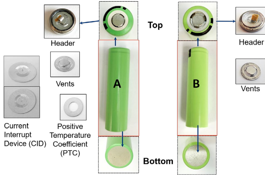
Figure 3. Photos showing the parts in the header of the cells from manufacturer A (OEM) and B (counterfeit). Destructive physical analysis (DPA) confirmed the presence of the safety devices PTC and CID in the high quality cells that were missing in the counterfeit cells.
