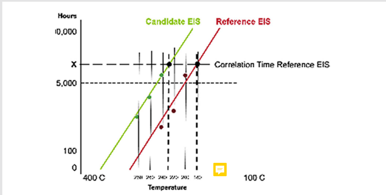
Figure 4: Insulation system life line analysis
